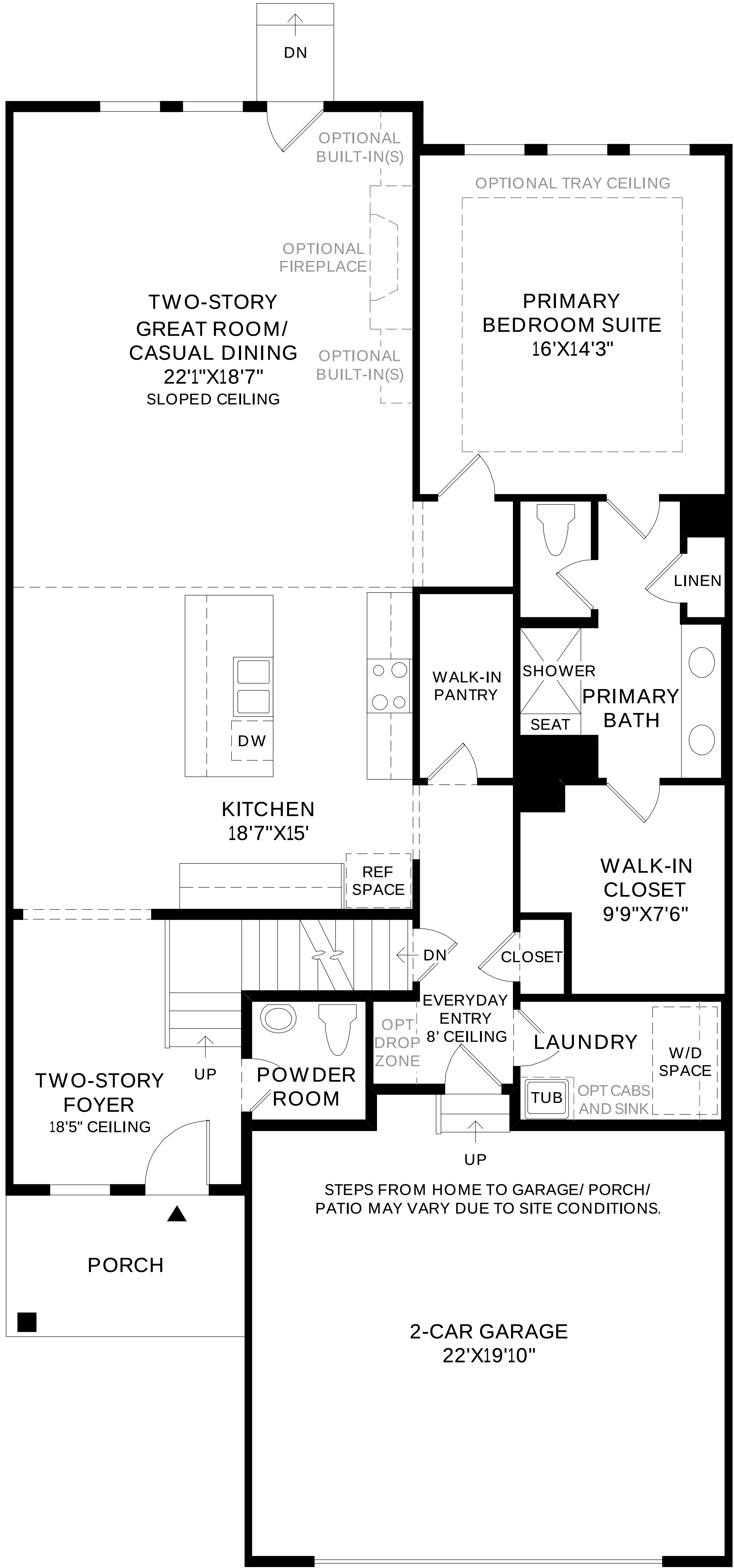
FIRST FLOOR 9' CEILING HEIGHT
